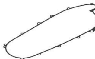
P018000004944 11395-K40-F00 CLUTCH COVER GASKET / JUNTA TAPA EMBRAGUE
